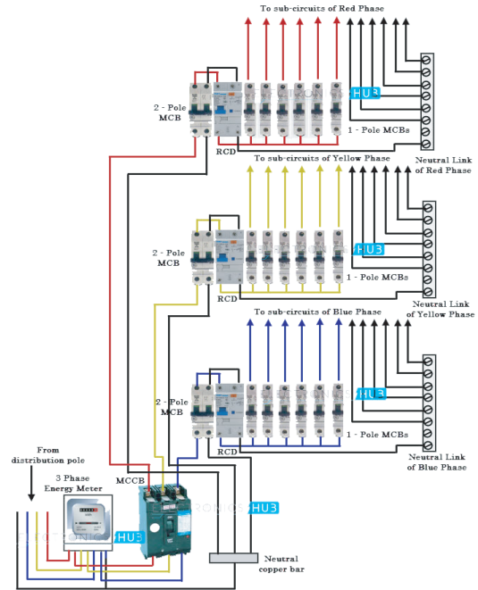
Three Phase Control Panel
